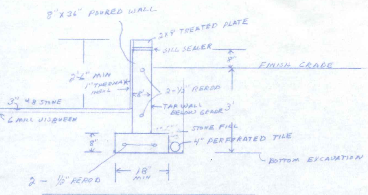
HOUSE FDN DETAIL GARAGE & PORCH FDN'S SAME EXCEPT 6" THICK & NO PERIMETER TILE
